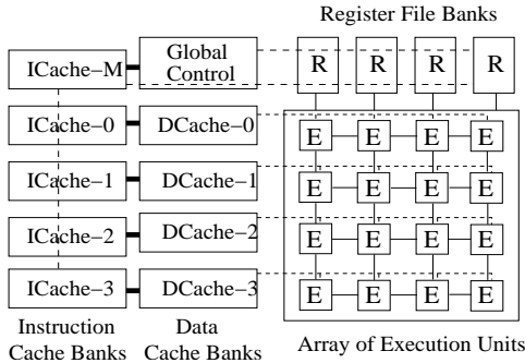
Fig. 1. TRIPS processor.
