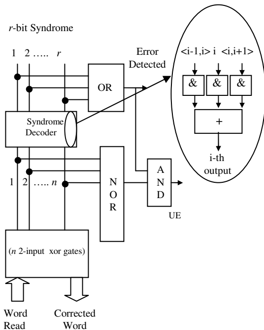
Figure 5. Error detection and correction block diagram
